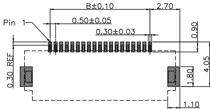
RECOMMEND PCB LAYOUT TOLERANCE:±0.05
