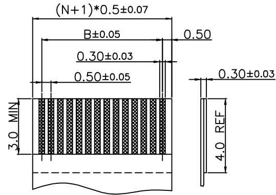
APPLICABLE FFC TOLERANCE:±0.05
