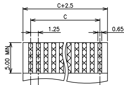
FPC/FFC T=0.30±0.05
