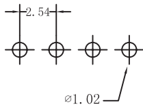
Recommended P. C. Board Hole Layout
