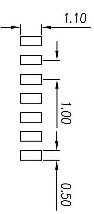
RECOMMENDED P.C. BOARD LAYOUT
